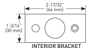
INTERIOR BRACKET
