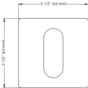
PREMIER SQ DEADBOLT INSIDE TRIM KIT
